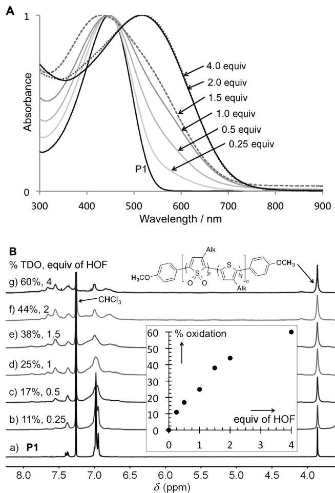
Figure 1. A) Normalized UV/Vis spectra (in chloroform) of P1 and its oxidized products obtained with increasing equivalents of HOF (0.25 to 4 equiv) per thiophene repeat unit. B) ^1\text{H} NMR spectra of P1 and its oxidized products, as the number of equivalents of HOF increased as follows: b) 0.25 equiv, c) 0.5 equiv, d) 1 equiv, e) 1.5 equiv, f) 2 equiv, g) 4 equiv; % TDO indicates the percentage of TDO units in the oxidized polymers. Inset: plot of the number of HOF equivalents vs. percent oxidation (i.e. % TDO units).
